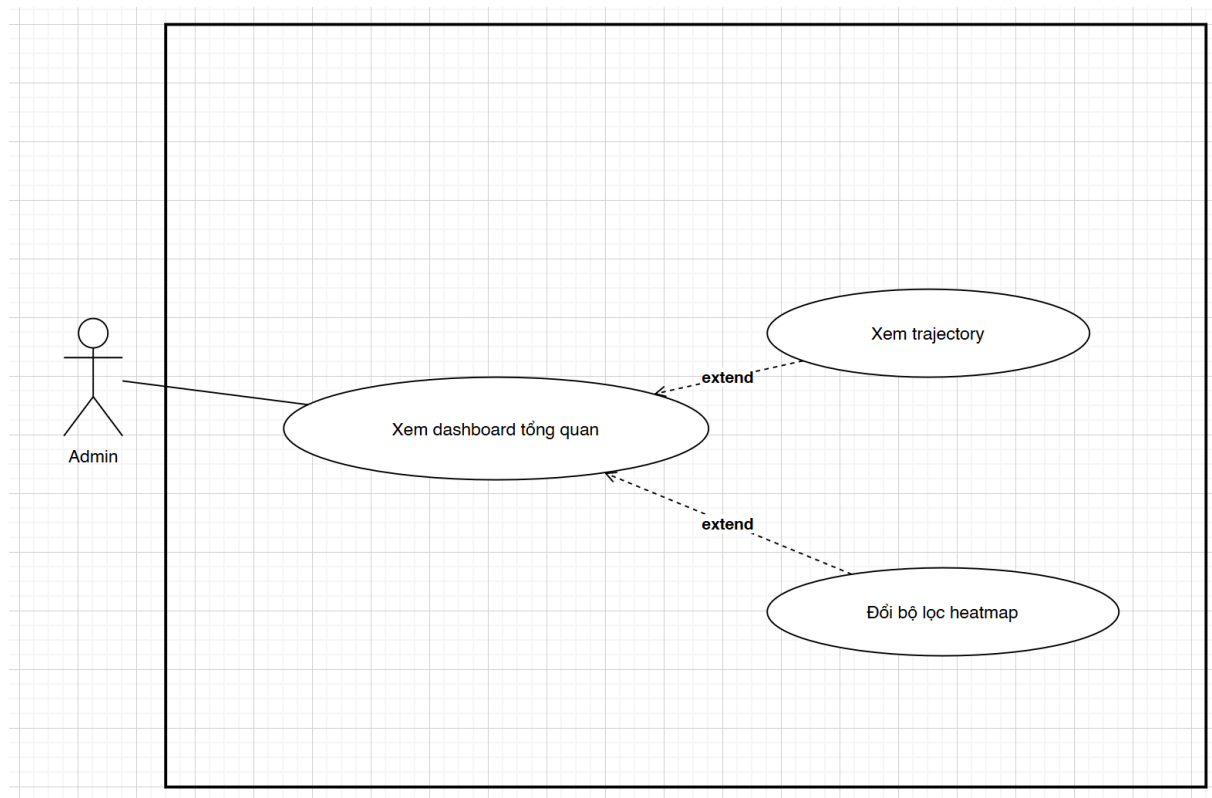
Dashboard.png
